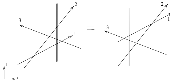
Figure 3. Pictorial representation of the generalized Yang–Baxter equation (44).
